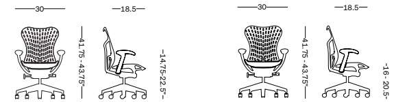
Work Chair with Butterfly Back
